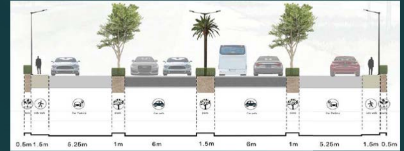
Front view
